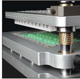
Blister Change Parts
