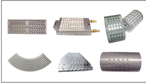
Blister Change Parts
